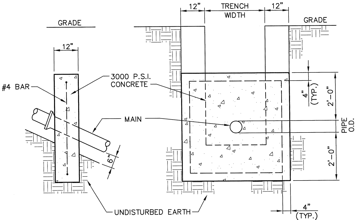
FRONT ELEVATION
