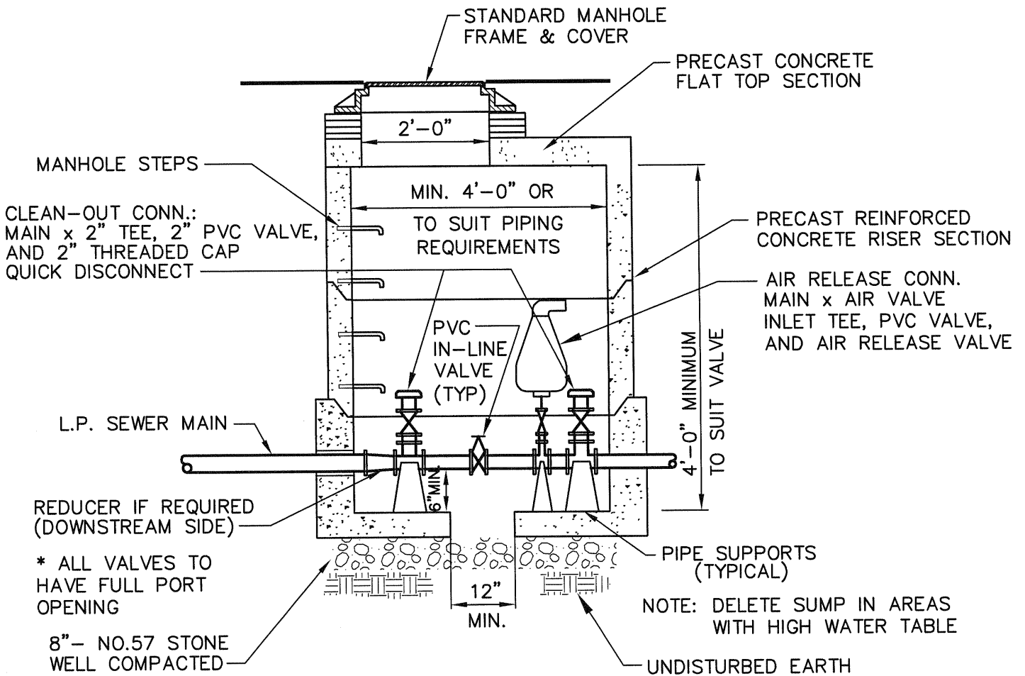
SECTION
