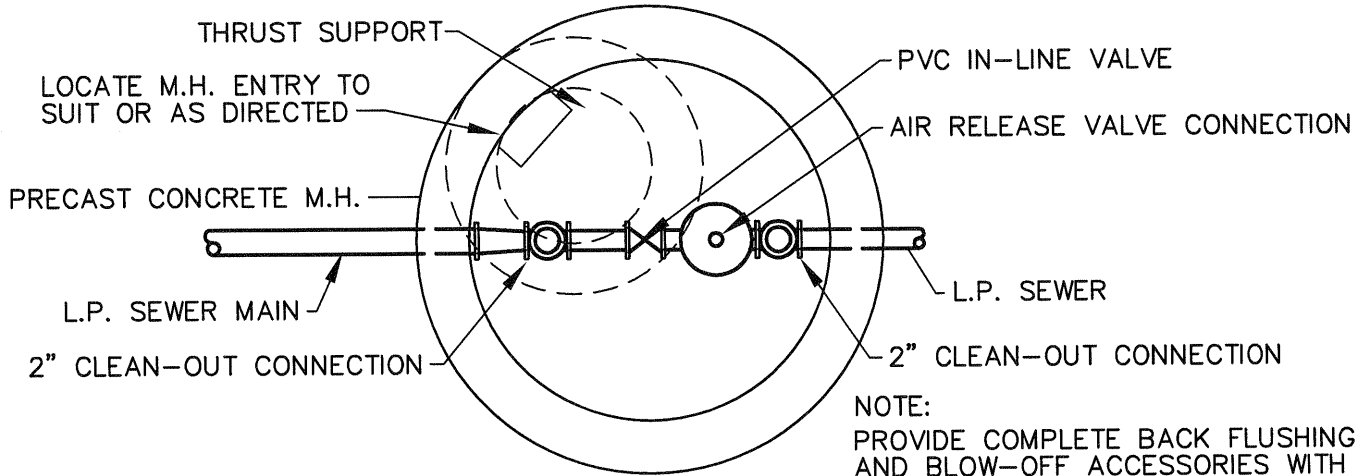
PLAN VIEW
